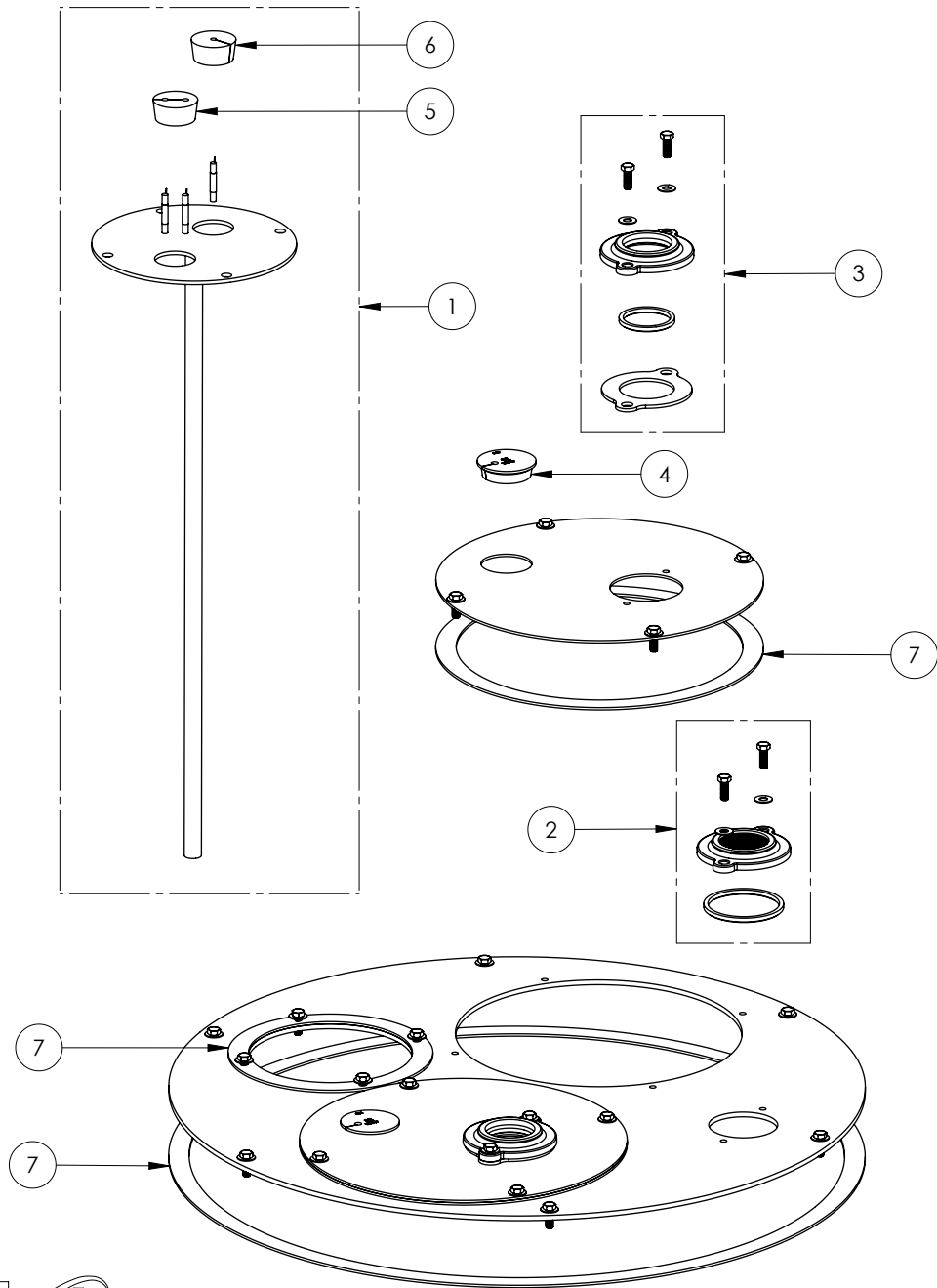
K001200 COVER KIT FOR 1100 SERIES 2" DISCHARGE AND 2" VENT
