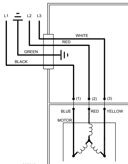
WIRING DIAGRAM FOR MODELS J404, F404, G404 AND BA404 ALL REVISIONS
