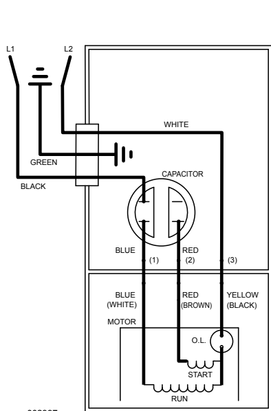
WIRING DIAGRAM FOR MODELS E404 AND I404 ALL REVISIONS
