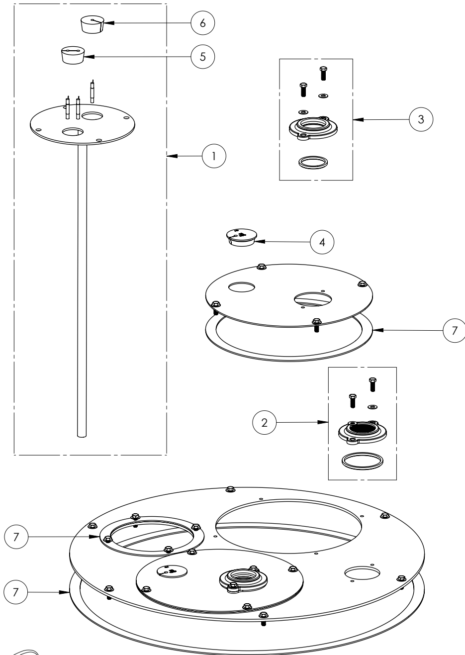
K001201 COVER KIT FOR 1100 SERIES 3" DISCHARGE AND 3" VENT
