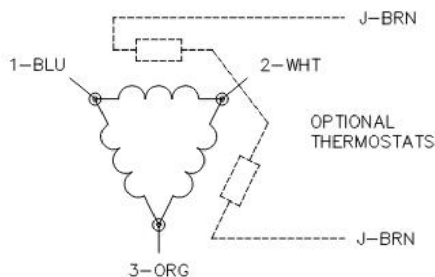
TYPICAL DELTA-CONNECTED MOTOR
