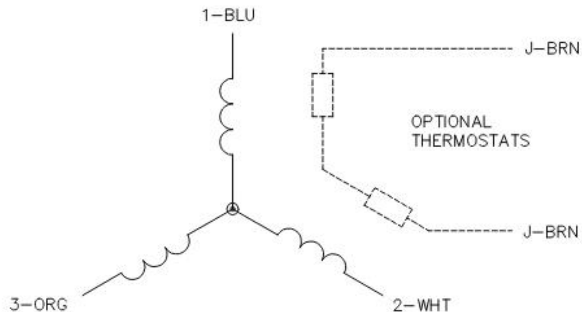
TYPICAL WYE-CONNECTED MOTOR
