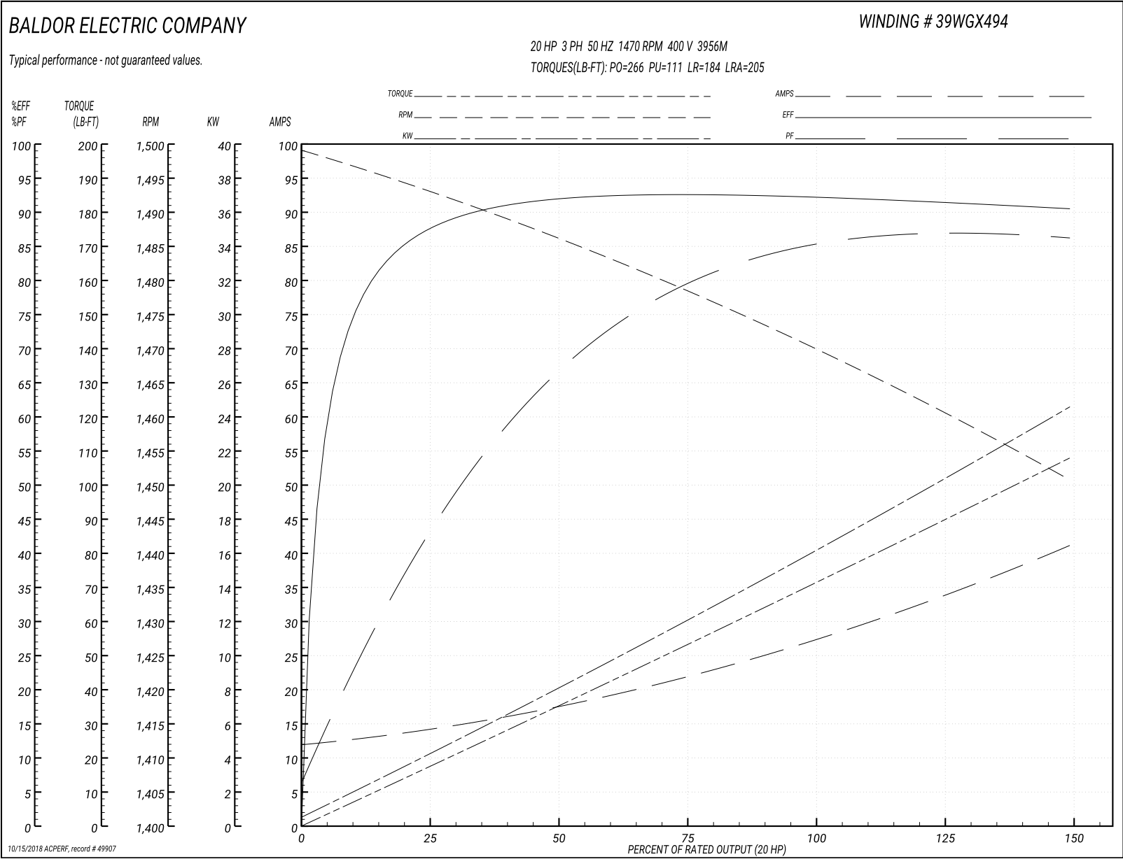
Performance Graph at 400V, 50Hz, 20.0HP Typical performance - Not guaranteed values
