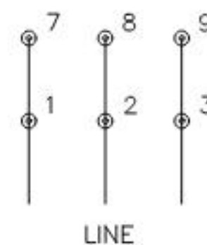
RUN CONNECTION
