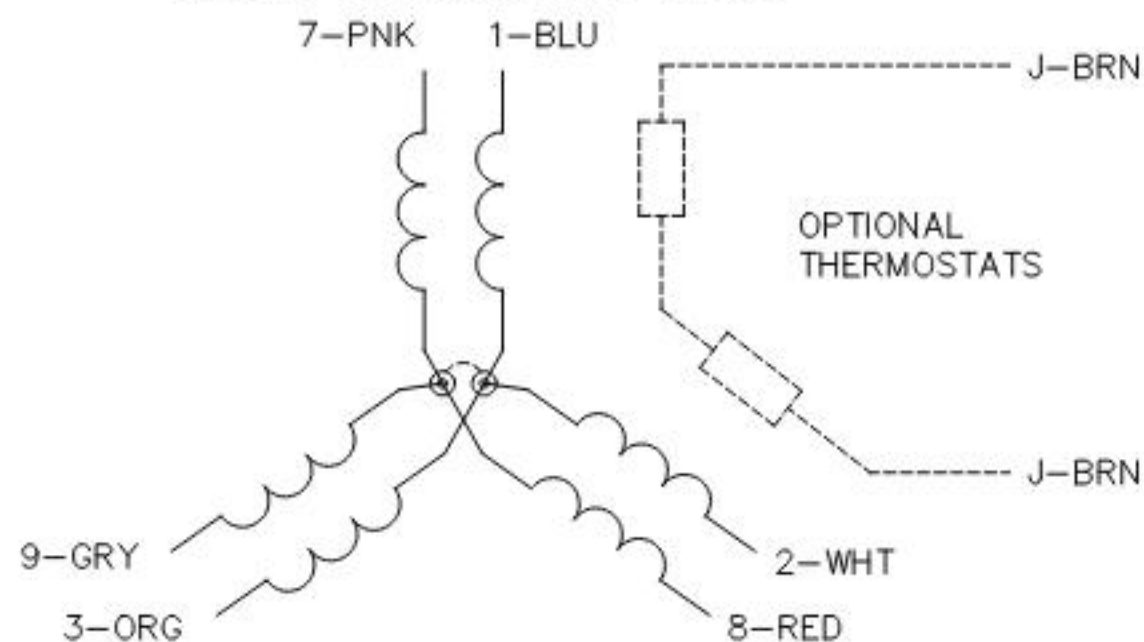
TYPICAL WYE-CONNECTED MOTOR
