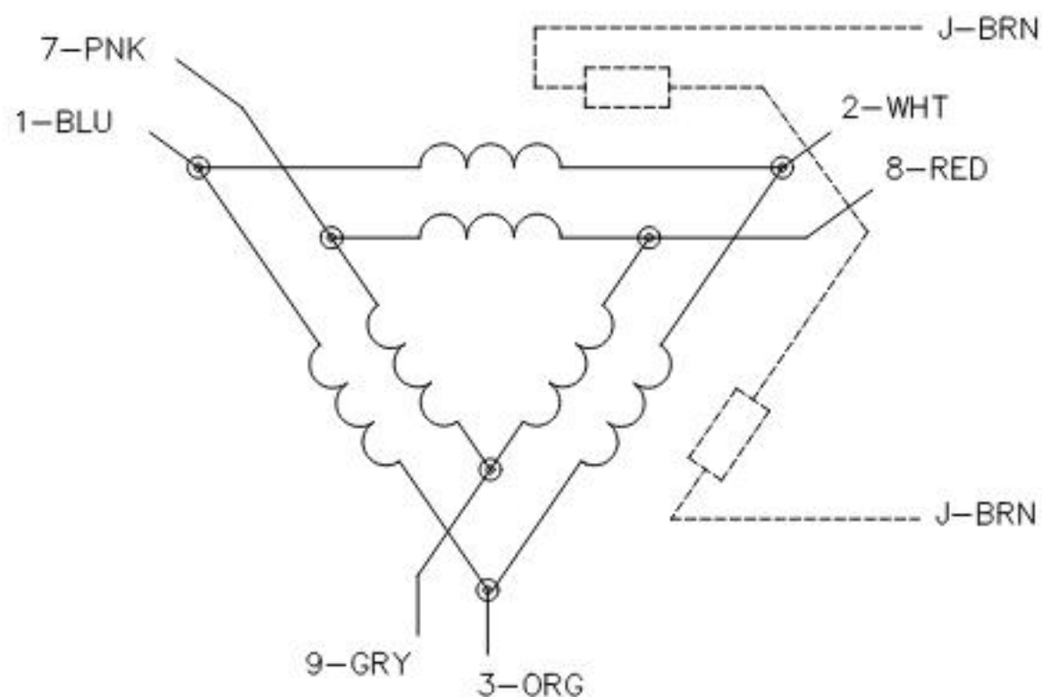
TYPICAL DELTA-CONNECTED MOTOR
