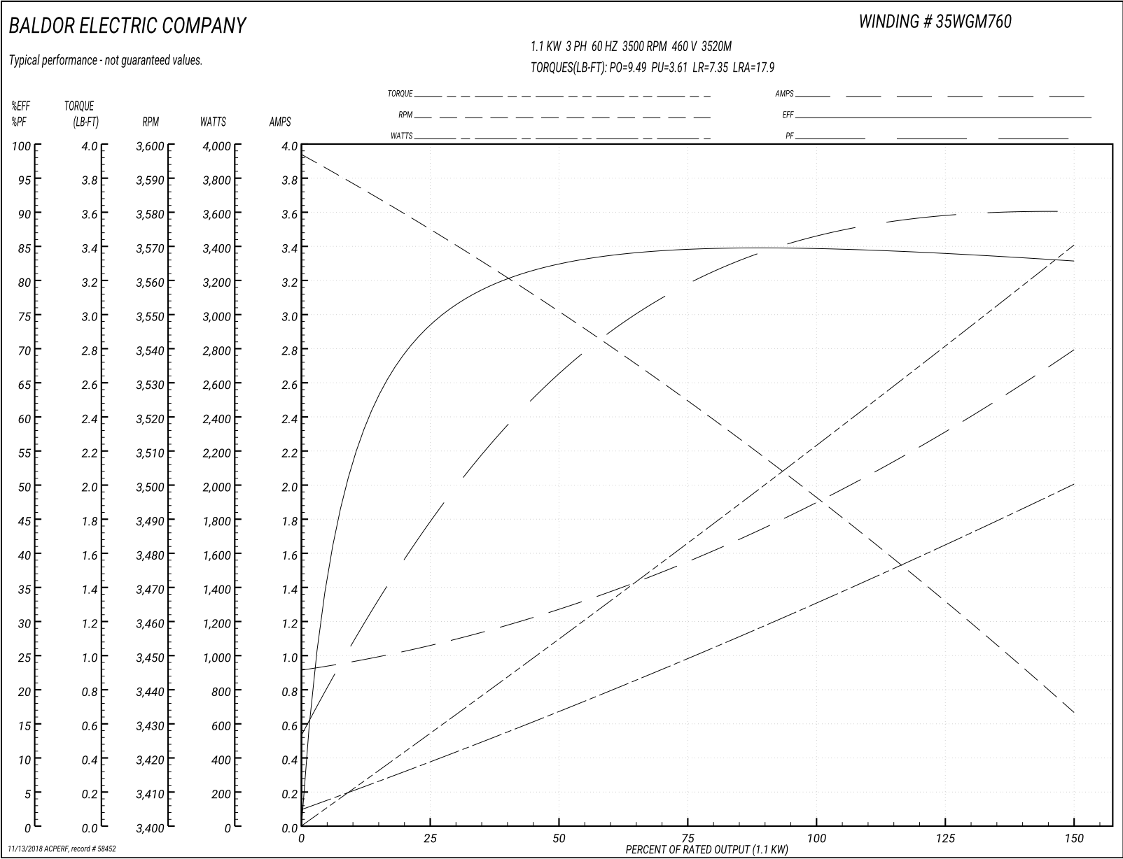
Performance Graph at 460V, 60Hz, 1.1KW Typical performance - Not guaranteed values
