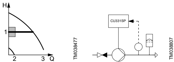
Constant pressure with stop function
