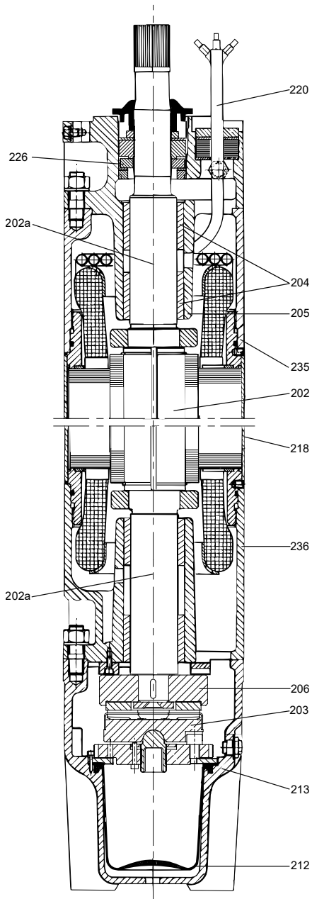
MMS 10000 motor
