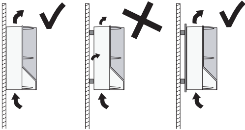
SmartFlo hung directly on the wall or fitted with a back plate
