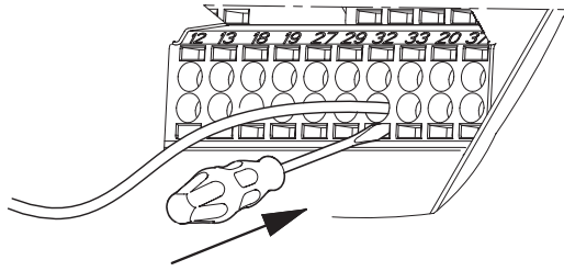
Fitting the conductor into the signal terminal
