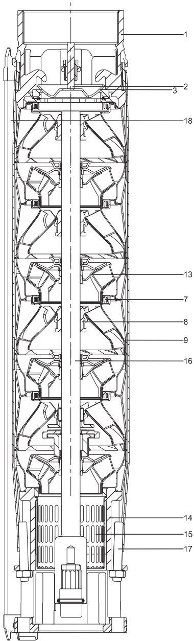
Example, SP pump, 6" (SP 90S - 300S)
