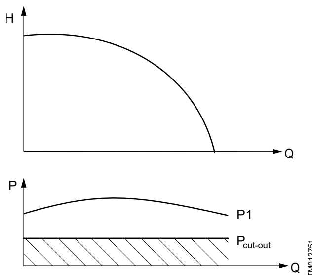
P_{\text{cut-out}} curve
