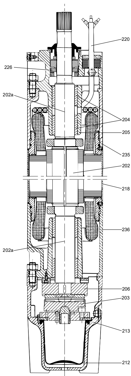
MMS 10000 motor
