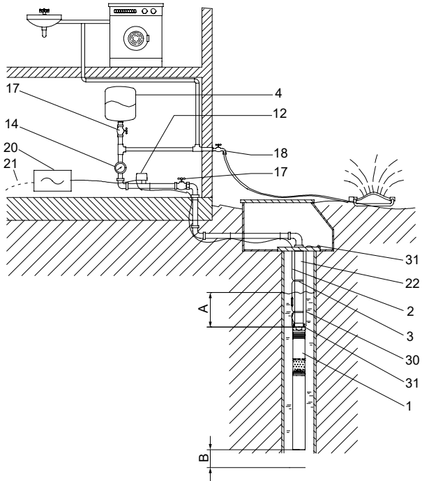
Application example: SQ with pressure switch and pressure tank
