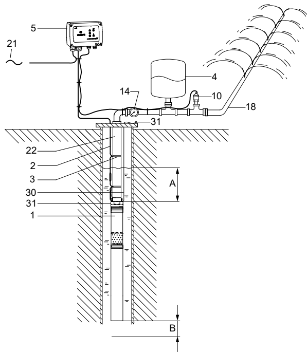
Application example: Constant-pressure control with CU 302 - irrigation
