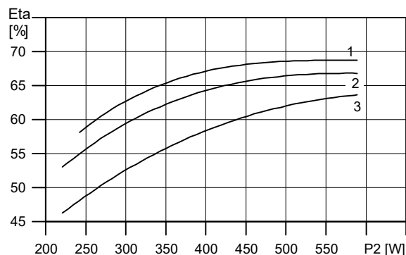
Efficiency curves of Grundfos SQ motor versus conventional motors
