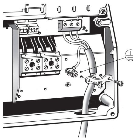
Motor connection
