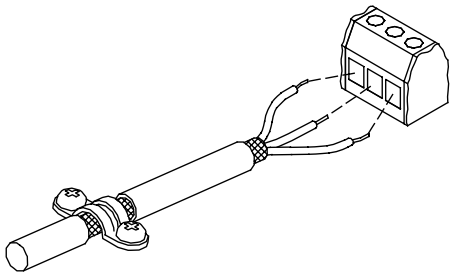
Example of stripped cable with screen
