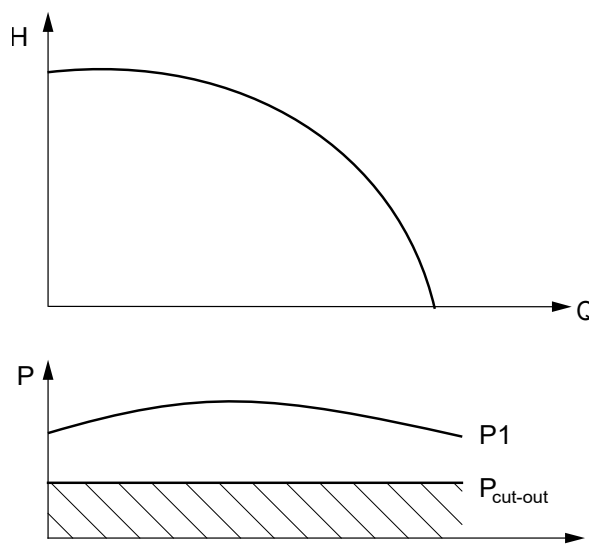
P_{\text{cut-out}} curve
