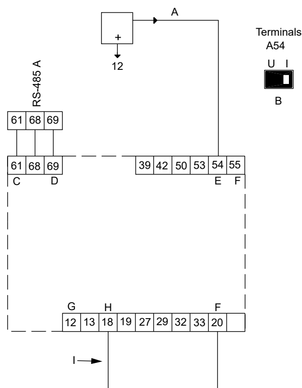
Wiring diagram for SmartFlo
