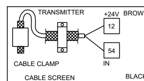
Sensor wiring diagram
