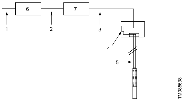
Example of installation in EMC-sensitive sites
