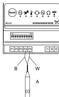
Connection to the IO 113
