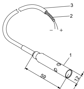
Water-in-oil sensor
