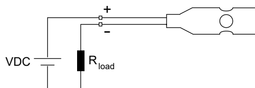
Connection of conductors
