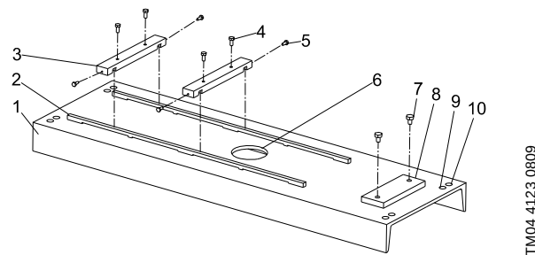
Fig. 11 Plaque de support Grundfos
