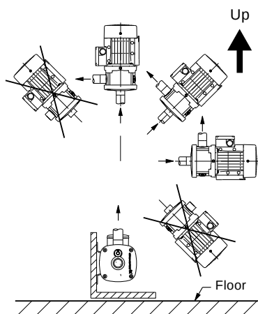
Fig. 4 Pump positions
