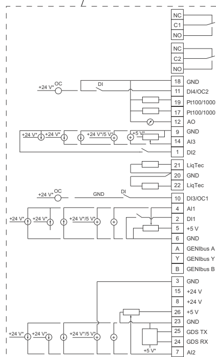
Fig. 4 Connection terminals, FM 300 functional module
