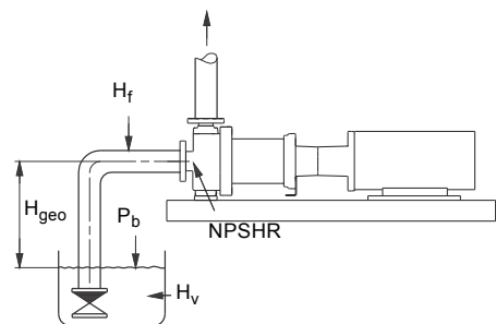
Fig. 52 Sizing data
