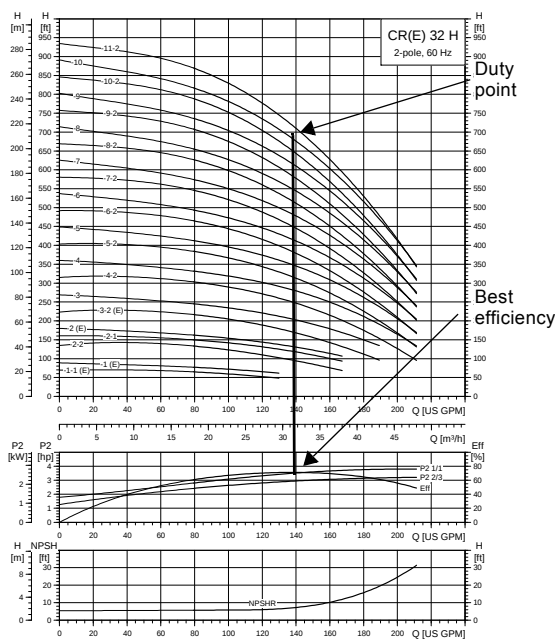
Fig. 53 Example of duty point
