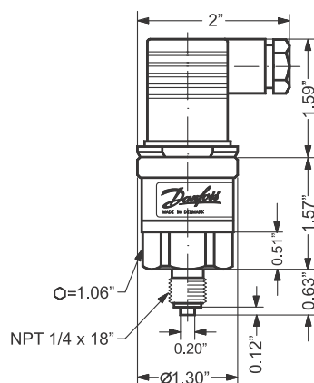
Fig. 67 Dimensional sketch
