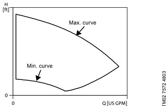
Fig. 55 Minimum and maximum performance curves
