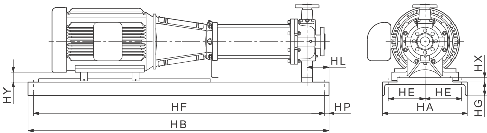
Baseplate dimensional sketch, CR(E), CRN(E) 32, 45, 64, 90 H
