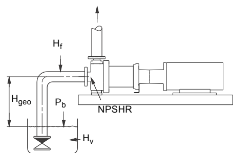
Fig. 52 Sizing data
