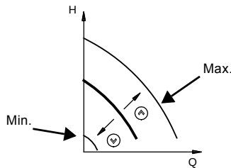
Fig. 24 Constant-curve mode
