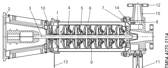
Fig. 46 Sectional drawing
