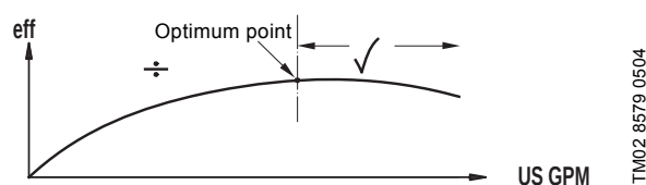
Fig. 54 Best efficiency
