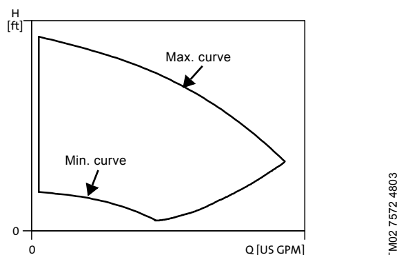
Fig. 55 Minimum and maximum performance curves
