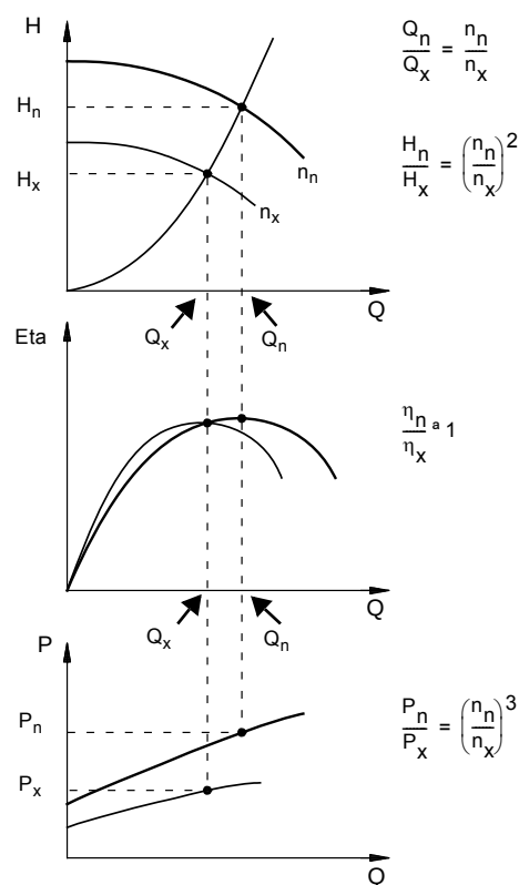
Fig. 56 Affinity equations
