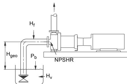
Fig. 52 Sizing data
