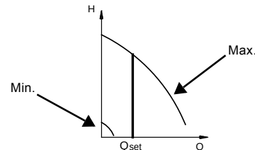
Fig. 25 Constant-flow mode
