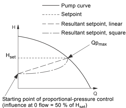
Fig. 16 Proportional-pressure control
