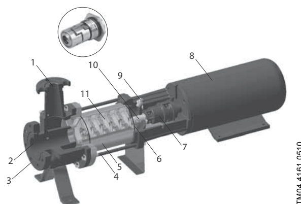
Fig. 3 CR-H pump
