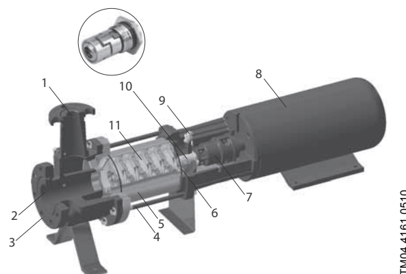
Fig. 3 CR-H pump
