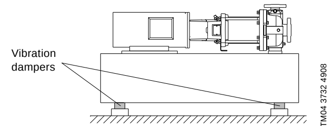
Fig. 9 Pump on vibration dampers
