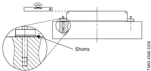
Fig. 8 Alignment with shims
