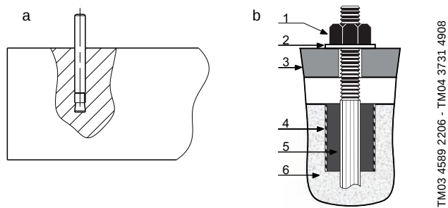
Fig. 7 Bolt in position (pos. a) and bolt sleeve detail (pos. b)
