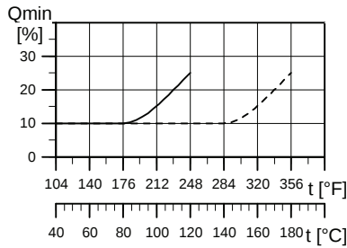
Fig. 5 Minimum flow rate
