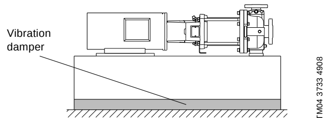
Fig. 10 Pump on vibration damper
