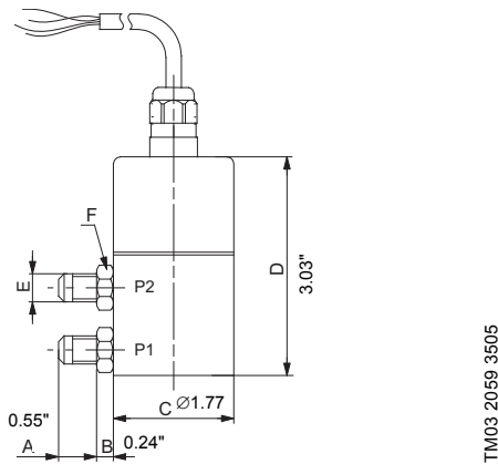
Fig. 69 Dimensional sketch
