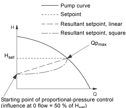
Fig. 16 Proportional-pressure control
