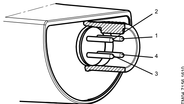
Fig. 73 Electrical connections
