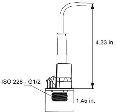
Fig. 66 Dimensions RPI transmitter
