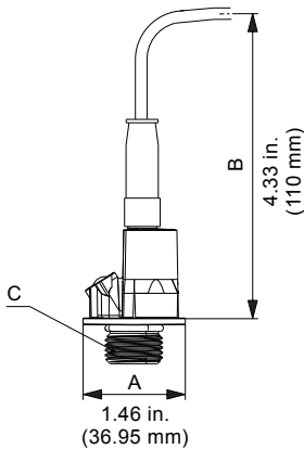
Fig. 71 DPI sensor g.2 version
