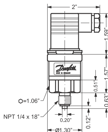
Fig. 67 Dimensional sketch
