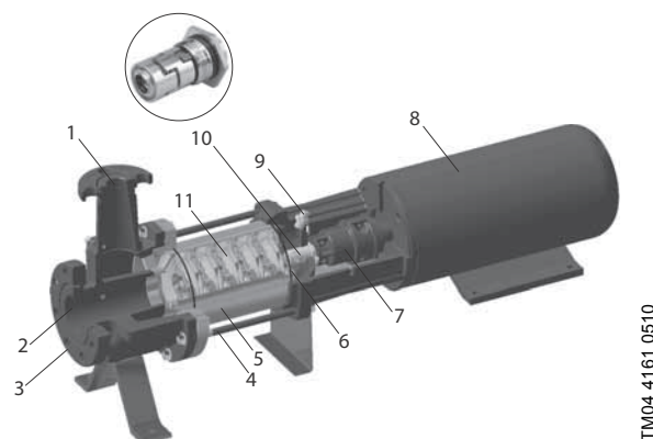
Fig. 3 CR-H pump
