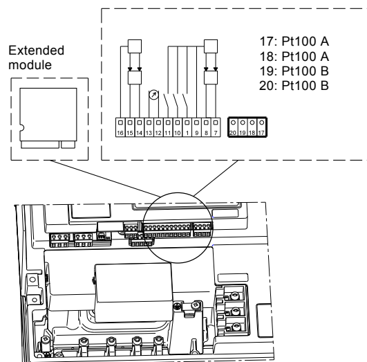
Fig. 29 Temperature sensor connections in the extended functional module
