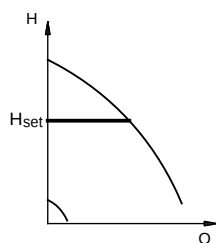
Fig. 23 Constant-pressure mode
