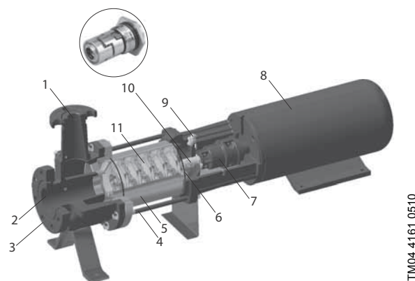
Fig. 3 CR-H pump
