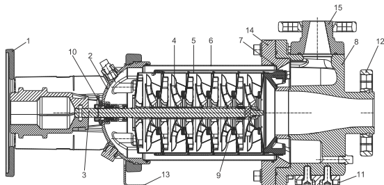
Fig. 44 Sectional drawing
