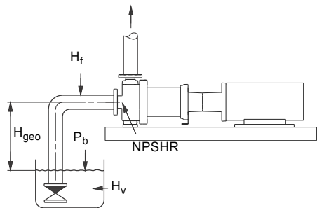
Fig. 52 Sizing data
