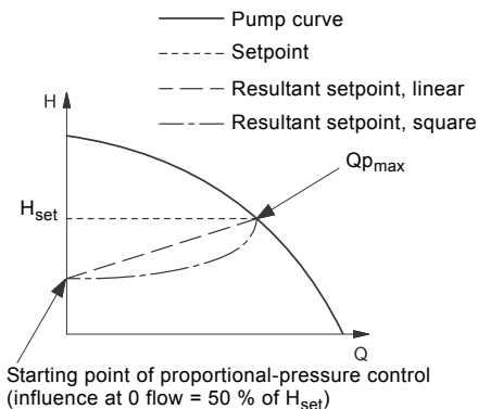
Fig. 16 Proportional-pressure control
