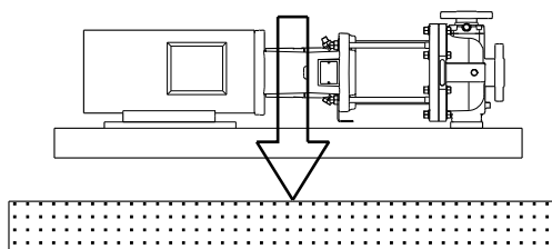
Fig. 6 Correct installation
