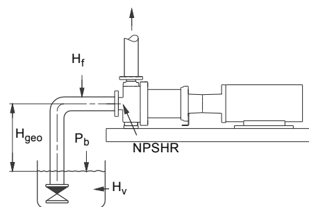
Fig. 52 Sizing data
