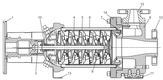
Fig. 42 Sectional drawing
