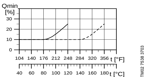
Fig. 62 Minimum flow rate
