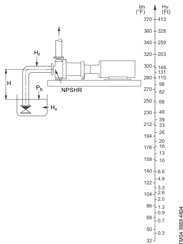
Fig. 60 Minimum inlet pressure - NPSHR
