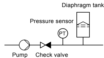
Fig. 27 Position of the check valve and pressure sensor in system with positive inlet pressure
