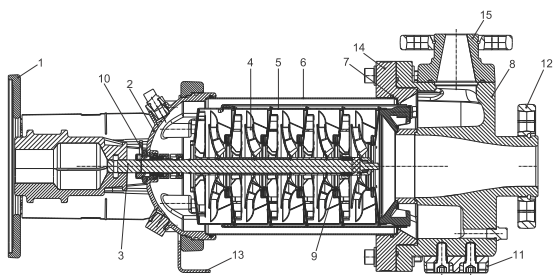
Fig. 44 Sectional drawing
