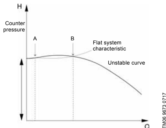
Fig. 39 Unstable pump curve
