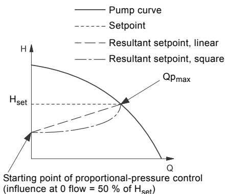
Fig. 16 Proportional-pressure control
