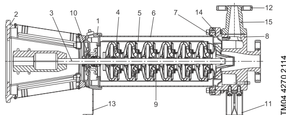
Fig. 48 Sectional drawing
