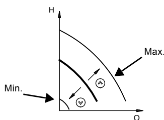
Fig. 24 Constant-curve mode
