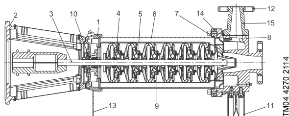
Fig. 46 Sectional drawing
