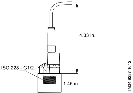
Fig. 66 Dimensions RPI transmitter
