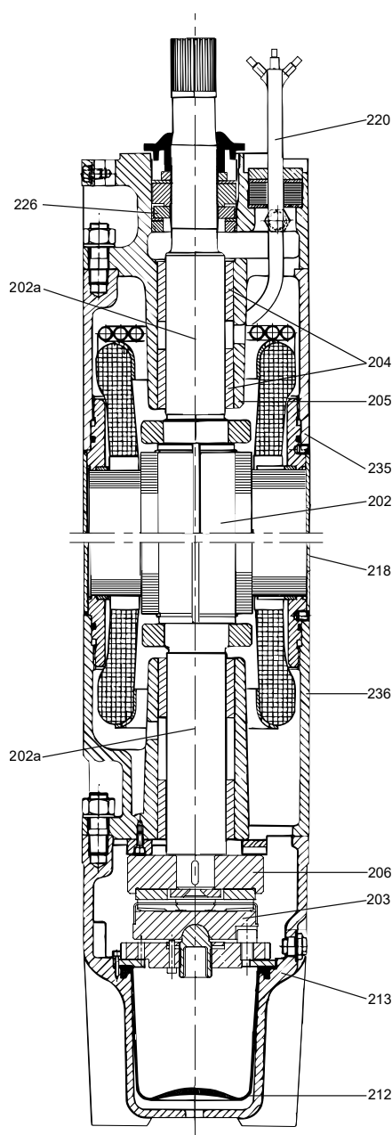
MMS 10000 motor
