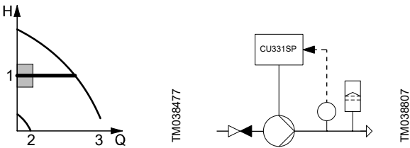
Constant pressure with stop function
