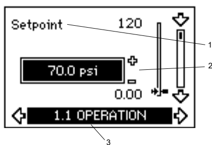
Example of display in the user menu
