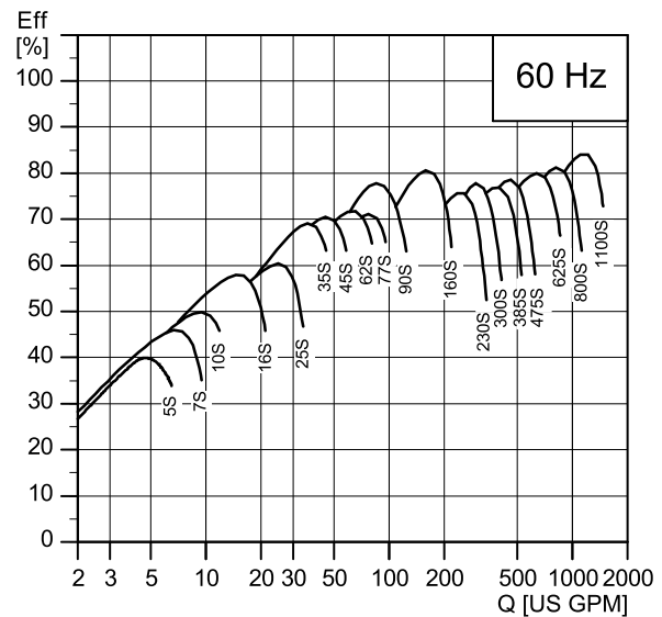
SP pump and motor efficiencies in relation to flow rate
