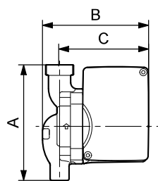
UP 15-10 BUC5, UP 15-10 BUC5/LC, UP 15-10 BUC5/TLC
