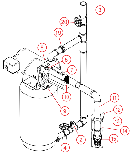
Shallow Well Tank Mounted System, Foot Valve
