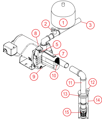
Shallow Well Tank Mounted System, Foot Valve
