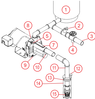
Shallow Well with Foot Valve
