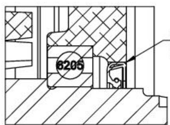
PULLEY END DETAIL
