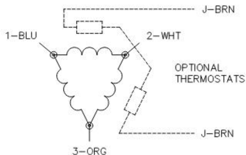
TYPICAL DELTA-CONNECTED MOTOR
