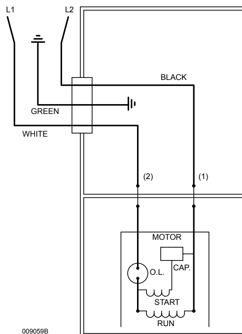
WIRING DIAGRAM FOR MODELS "BN2098-A" and "BN2098-B" "BE2098-A" and "BE2098-B" 02/01 thru Current
